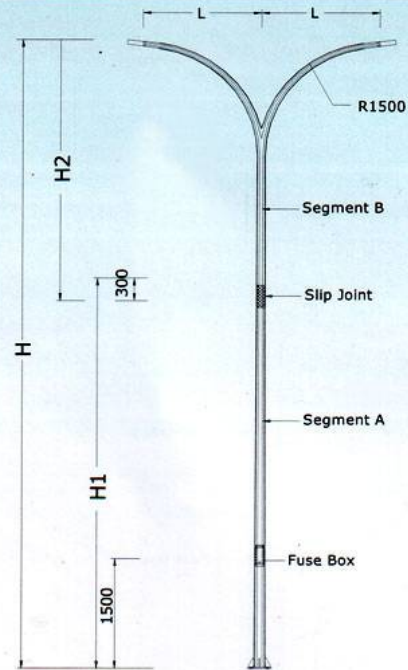
DOUBLE TYPE PARABOLA
