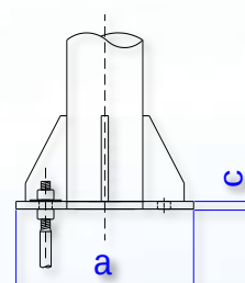
BASE PLATE Side view
