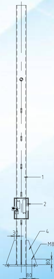
FRONT VIEW
