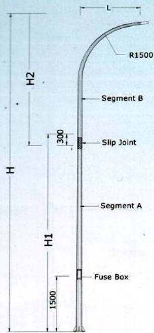
SINGLE TYPE PARABOLA
