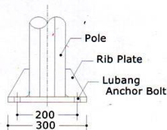
POT. BASE PLATE
