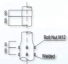
JOINT
