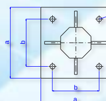
BASE PLATE
