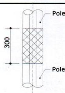
SLIP JOINT
