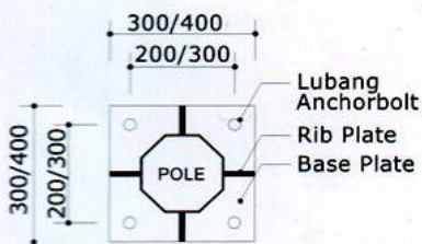
BASE PLATE
