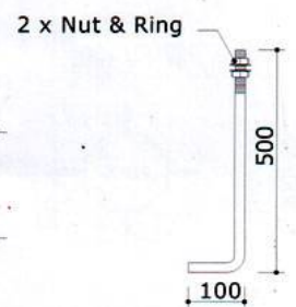
ANCHOR BOLT
